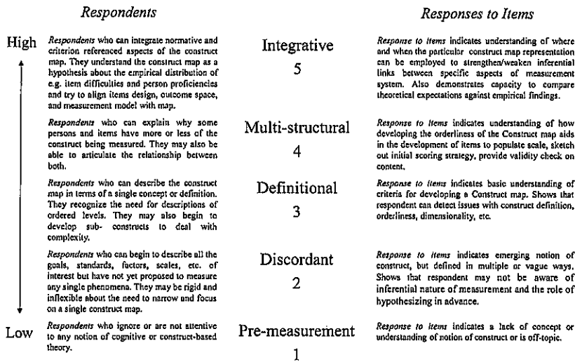
Figure 3. Construct map for UCM variable.
