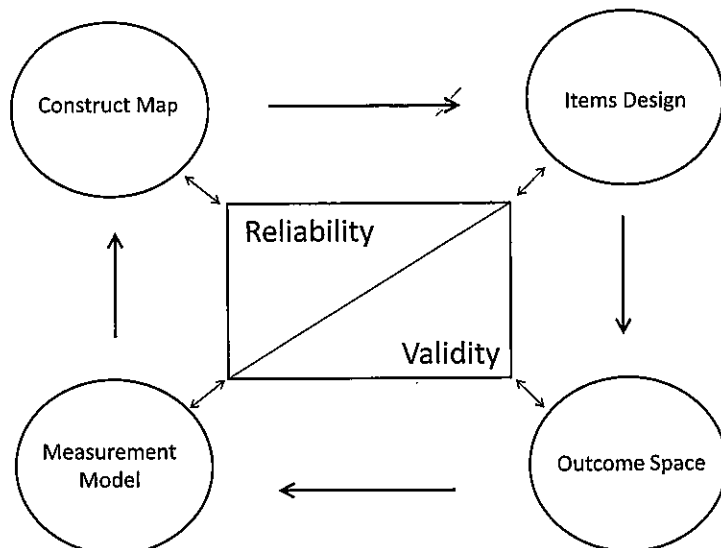
Figure 2. Relations among topics of CM knowledge.
